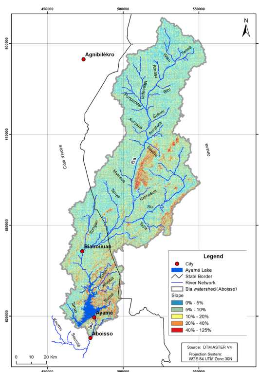
Fig 5 Slope spatial distribution of Bia watershed upstream Aboisso.
