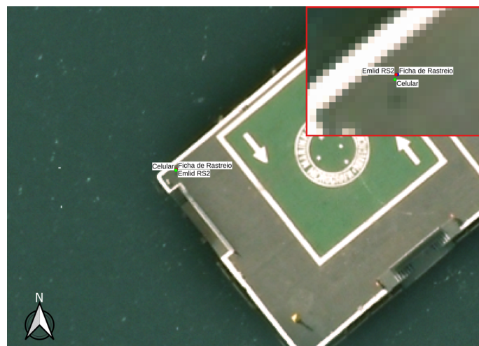
Fig. 8 Plotted coordinates of the MT Pier of the DHN using the ONRJ as a reference station. Source: Adapted from QGIS (2022).
