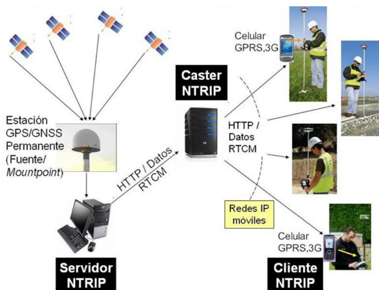
Fig. 4 NTRIP operating structure. Source: Giovanni (2021).
