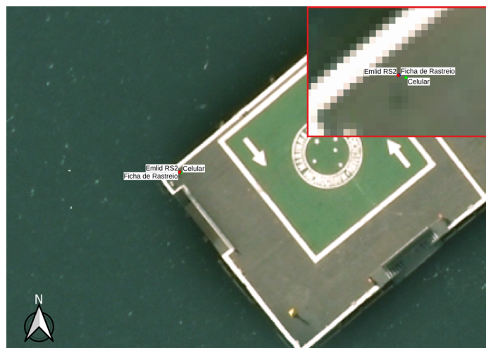
Fig. 7 Plotted coordinates of the MT Pier of the DHN using the RJNI as a reference station. Source: Adapted from QGIS (2022).
